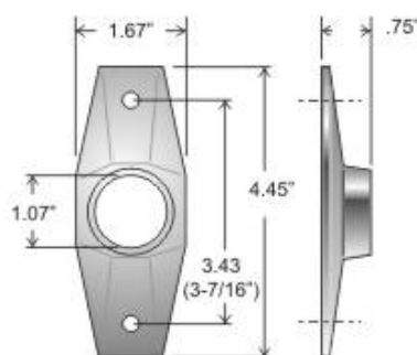
Mounting flange, front and side views
