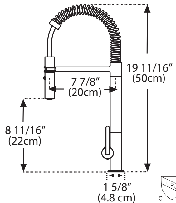
Dimensional Drawing
