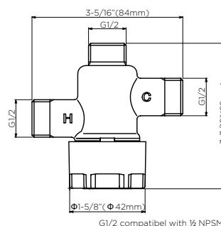
Thermostatic Mixing Valve (TLT10)
